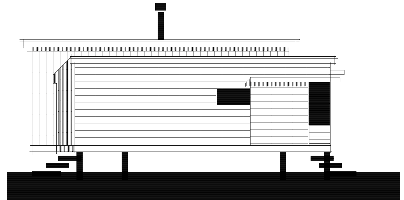
PAYILLON No.1 ELEVATION GAUCHE
