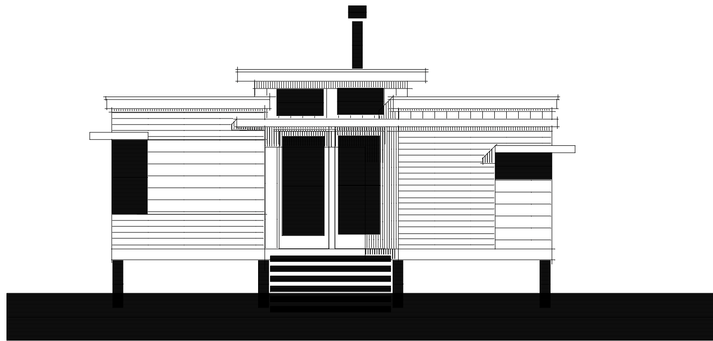
PAYILLON No.1 ELEVATION AVANT
